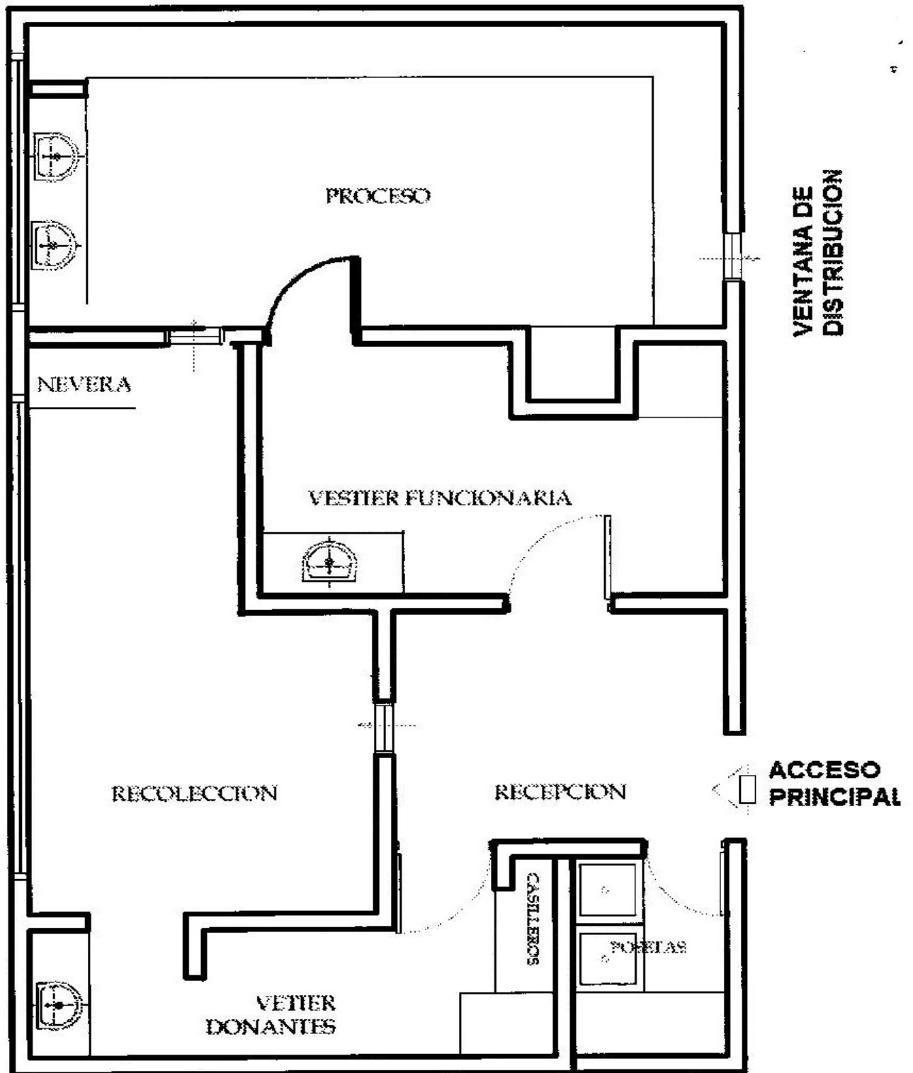
BANCO DE LECHE HUMANA HOSPITAL SAN RAFAEL FUSAGASUGA
